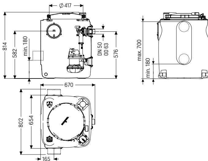
Illustration shows.: Art. no. 28 518
