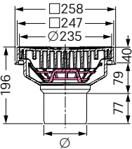
Illustration shows Art. no. 67 110B
