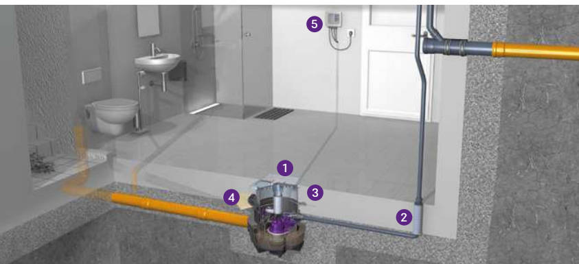
1 Lifting station 2 Pressure pipe set 3 Extension section 4 Gasket set 5 Control unit
