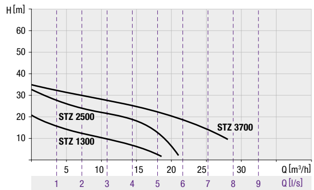
Pump STZ 1300, STZ 2500 and STZ 3700
