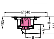
Ø 78 Art. no. 48 578
