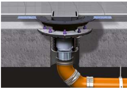
Shallow and lower waterproofing flange
