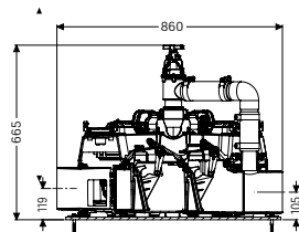
Illustration shows Ecolift L Duo SWA
