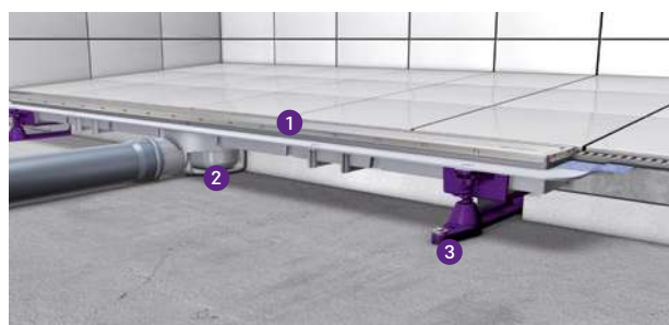
1 Channel cover 2 Drain body 3 Installation supports
