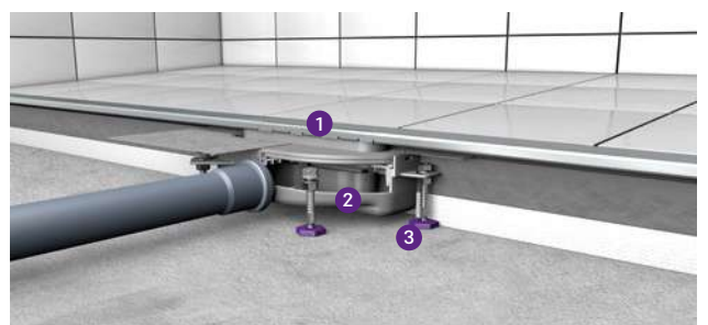
① Channel cover ② Drain body ③ Installation supports
