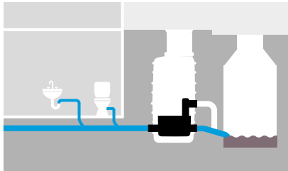
Hybrid lifting stations make use of the natural slope to the sewer.
