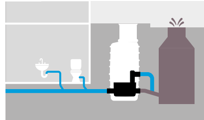
The building's wastewater is pumped into the surcharged sewer during times of backwater.
