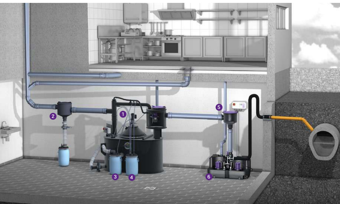
1 Grease separator 2 Pre-filter 3 Sludge storage tank 4 Grease storage tank 5 Sampling chamber 6 Lifting station
