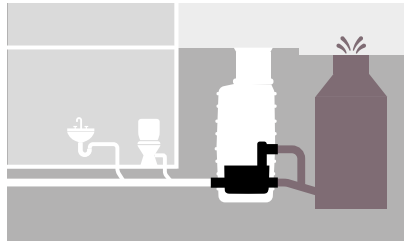
Motorised flap(s) close to prevent backwater from entering from the surcharged sewer.
