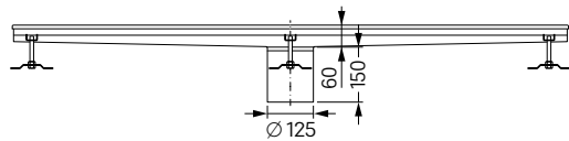
Illustration shows B = 153 mm
