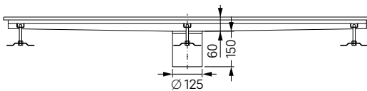
Illustration shows B = 200 / 300 / 400 mm
