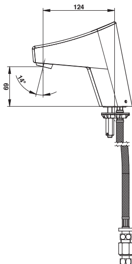
SINGLE DECK-MOUNTED TAP
