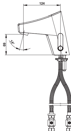
DECK-MOUNTED MIXER TAP
