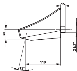
SINGLE WALL-MOUNTED TAP
