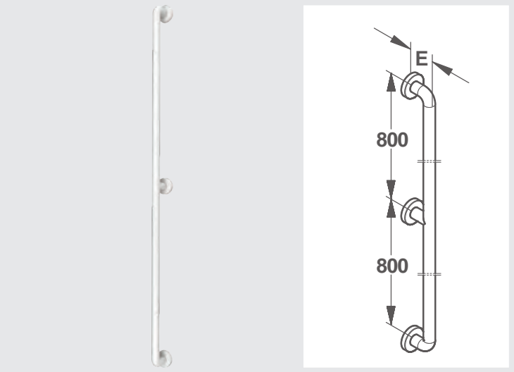
Ø 34 mm VERTICAL RAIL
