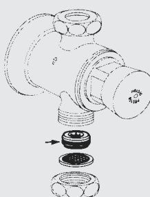
Flow regulator (Models pre-March 1989)
