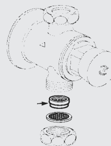
Flow regulator (Models starting from March 1989)
