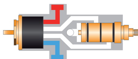
Mixer tap in closed position NO CONTAMINATION POSSIBLE
