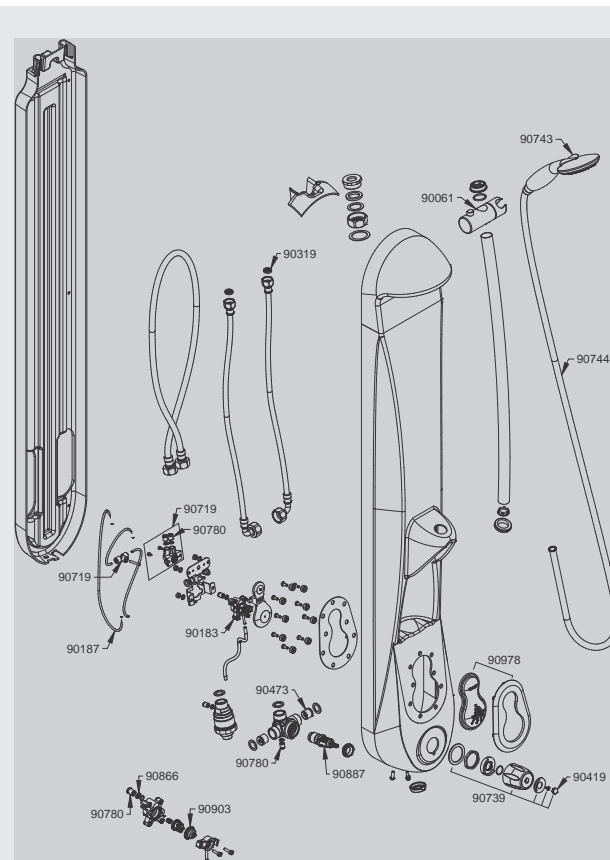
DL 800 S® WITH HAND-HELD SHOWER
