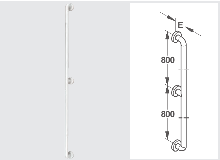
Ø 35 mm VERTICAL RAIL
