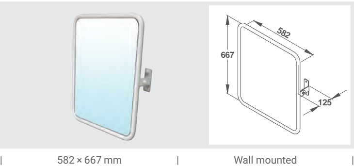
TILTING MIRROR
