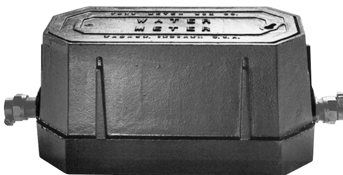
Long Gulfboxes for 5/8"x3/4" Meter with Cartridge Dual Check Valve
