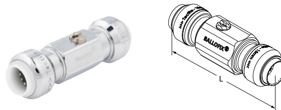
Ballofix® without handle (2 × push)
