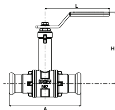
XPress® full flow press valve with handle, long stem (2 × press)
