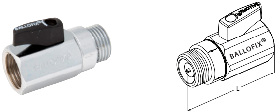
Ballofix® with non-return valve and handle (female x male)
