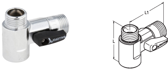
Ballofix® tee with non-return valve and handle, without shut-off (female x male)
