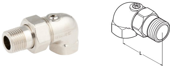
Ballofix® angled radiator tail piece (female x male)
