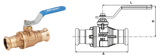
XPress® full flow press valve with handle, short stem (2 × press)
