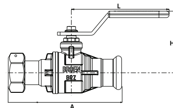
XPress® full flow press valve with handle, short stem (swirvel nut × press)
