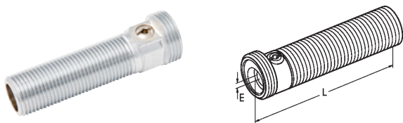
Ballofix® eccentric tail piece, long model (2 × male)
