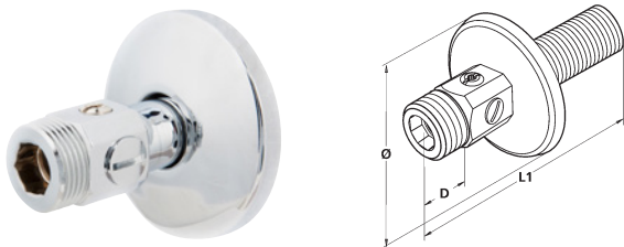
Filterfix® straight valve with flange, without handle (2 × male)
