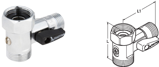
Ballofix® tee with non-return valve and handle (male x swivel nut)
