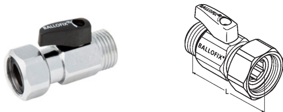
Ballofix® with handle (swirvel nut x male)
