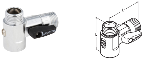
Ballofix® tee with non-return valve and handle (female x male)
