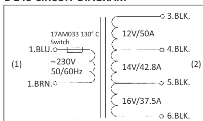
E-248 CIRCUIT DIAGRAM
