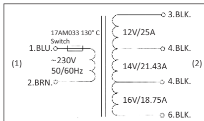
E-246 CIRCUIT DIAGRAM
