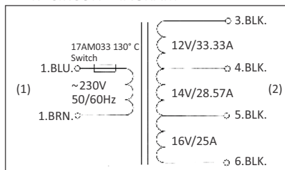
E-247 CIRCUIT DIAGRAM
