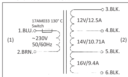
E-245 CIRCUIT DIAGRAM
