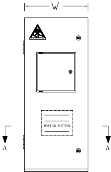
FRONT ELEVATION
