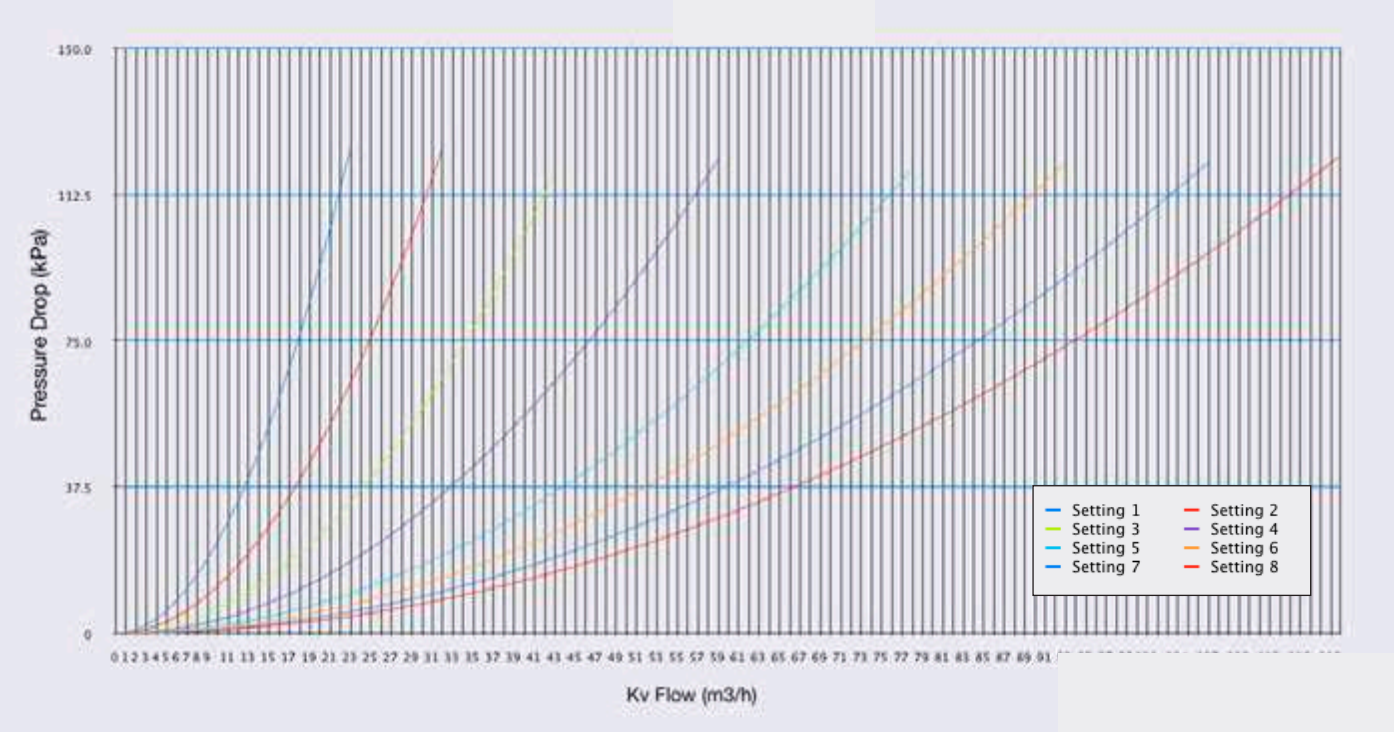
DN80 V952 - Variable Orifice Double Regulating Valve
