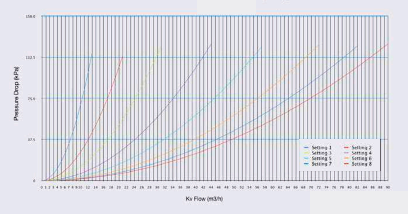
DN65 V952 - Variable Orifice Double Regulating Valve
