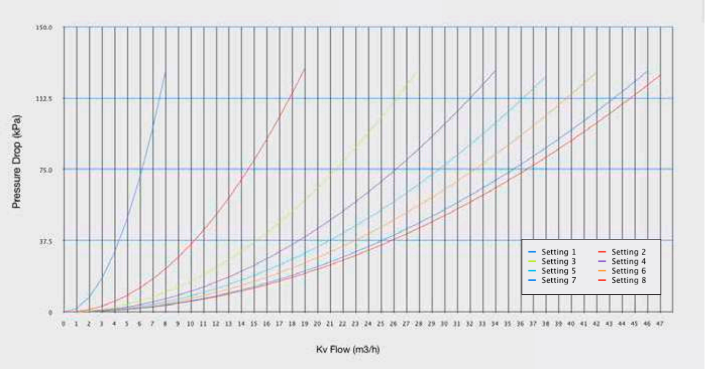
DN50 V952 - Variable Orifice Double Regulating Valve
