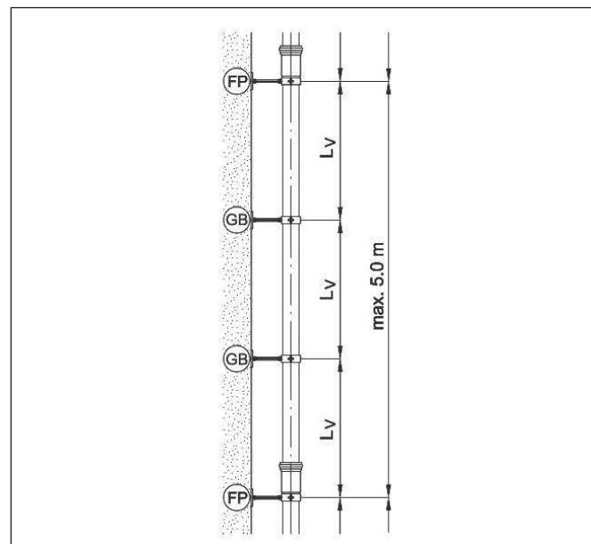
Illustration 7.8 Vertical installation
